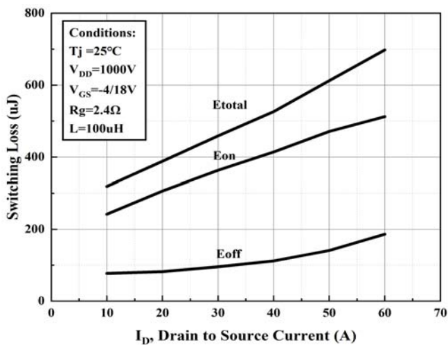
Figure 19. Clamped Inductive Switching Energy vs. Darin Current
