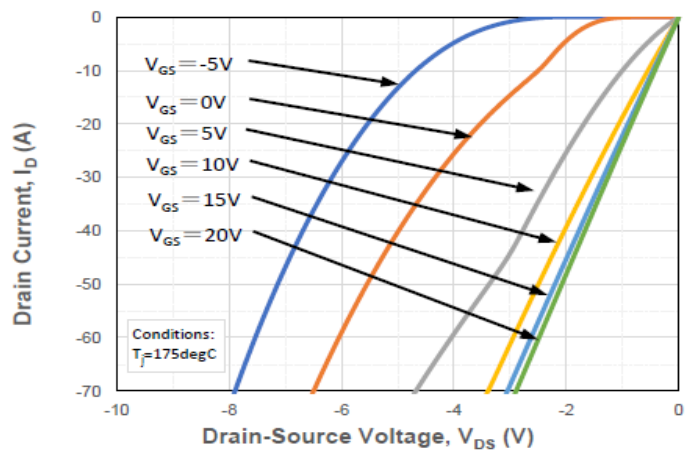
Figure 9. Reverse Output Characteristics at Tj = 175°C
